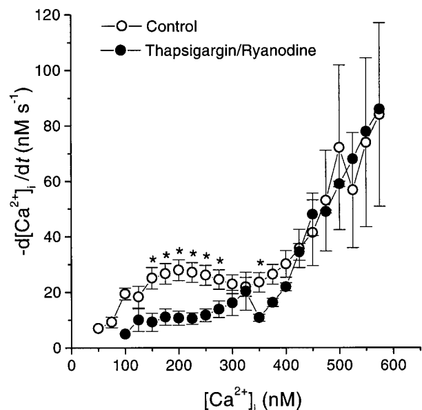
FIGURE 4 Comparison of the rate of \text{Ca}^{2+} removal as a function of [\text{Ca}^{2+}]_i in the absence or presence of thapsigargin or ryanodine. The third phase removal rate was significantly ( p < 0.05 ) faster in control cells than in those treated with store \text{Ca}^{2+} uptake inhibitors, as shown by *.
