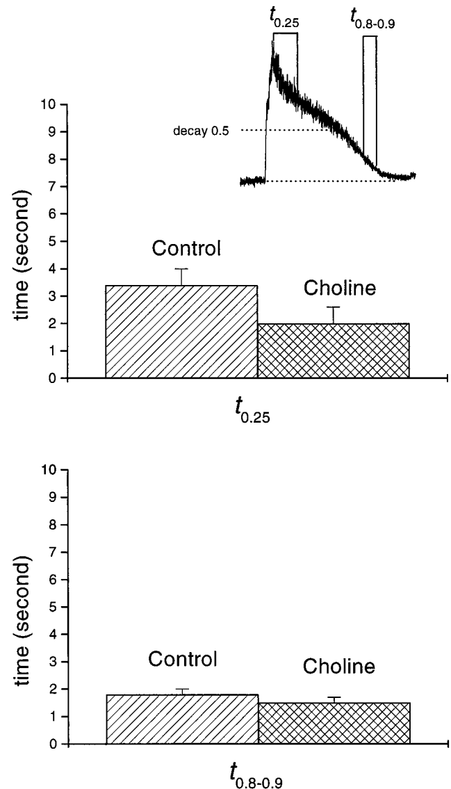
FIGURE 6 Comparison of t_{0.25} and t_{0.8-0.9} in the Na + -containing (control) and Na + -free choline + -bathed cells. The inhibition of the Na + -Ca 2+ exchanger did not affect either t_{0.25} or t_{0.8-0.9} . The inset illustrates t_{0.25} and t_{0.8-0.9} .
